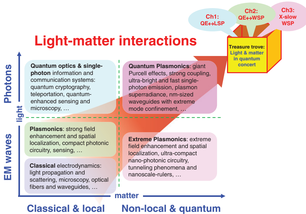
Figure 1: Quantum aspects of plasmonics exhibit both in the quantum nonlocal response of matter and in the quantized light fields. With the developments of quantum plasmonics, we anticipate a “treasure trove” of emerging quantum technologies that harvest from the quantum concert of both light and matter. In the main text, we outline three challenges associated with this.
